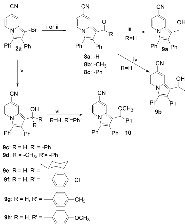
Scheme 2. Reagents and conditions: (i) (1) BuLi, THF, -78 °C; (2) DMF or PhCOCl; (ii) Bu 3 SnC(Oet)=CH 2 , cat Pd(0), DMF, 100 °C; (iii) NaBH 4 , EtOH; (iv), CH 3 Li, -78 °C, THF; (v) BuLi, THF, -78 °C; (2) RCOR'; (vi) NaH, CH 3 I, THF.
