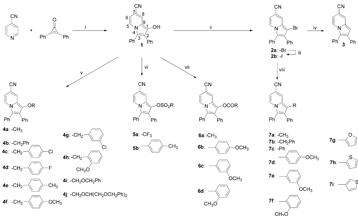
Scheme 1. Reagents and conditions: (i) DCE, \Delta ; (ii) Br 2 , PPh 3 , MeCN, 70 °C; (iii) (1) BuLi, THF, -78 °C; (2) I 2 ; (iv) (1) BuLi, THF, -78 °C; (2) NH 4 Cl(aq); (v) NaH, alkyl halide, THF; (vi) TsCl/0 °C or Tf 2 O/-78 °C, DMAP, CH 2 Cl 2 ; (vii) (RCO) 2 O or RCOCl, DMAP, DCE; viii, RSnBu 3 , RZnX or RB(OH) 3 , cat Pd(0), 60–100 °C, dioxane or DMF.
